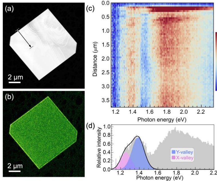
Figure 4. STEM cathodoluminescence spectroscopy of homogeneous SnS flakes. (a) HAADF-STEM image of a large, homogeneous SnS flake (edge length: 9.2 \mu\text{m} , thickness \sim 150 nm; see Supporting Figures 5 and 6). (b) Panchromatic STEM-CL map of the flake shown in (a). (c) Hyperspectral CL linescan along the arrow in (a). (d) CL spectrum obtained within the SnS flake ( >3 \mu\text{m} from the edge). Colored peaks: Gaussian lineshape analysis of the contributions of the SnS X-valley (pink) and Y-valley (blue) to the low-energy light emission.
