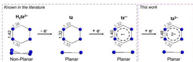
Fig. 2 Comparison of the metric parameters of the different tetrazine species. The metric parameters for the doubly deprotonated dihydrotetrazine have been extracted from [(\text{Cp}_2\text{Ti}(\mu\text{-H}_2\text{tz}^{2-}))_4] , 81 while the metric parameters for the neutral \text{tz} have been extracted from [\text{Ag}(\text{tz})(\text{NO}_3)]_n . 36
