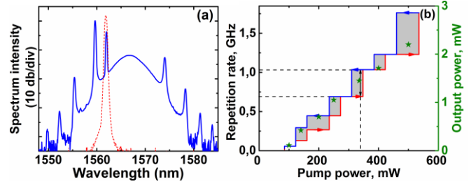
Fig. 2. Laser optical spectra recorded at a pump power of ~40 mW (CW operation, red dotted line) and 450 mW (HML soliton trains, PRR~1.23 GHz, blue solid line) (a). PRR as a function of the increasing (red line) and decreasing (blue line) pump power. The PC settings are fixed. The grey areas show the PRR range subjected for the PRR precise setting. Green asterisks show the output power (b).
