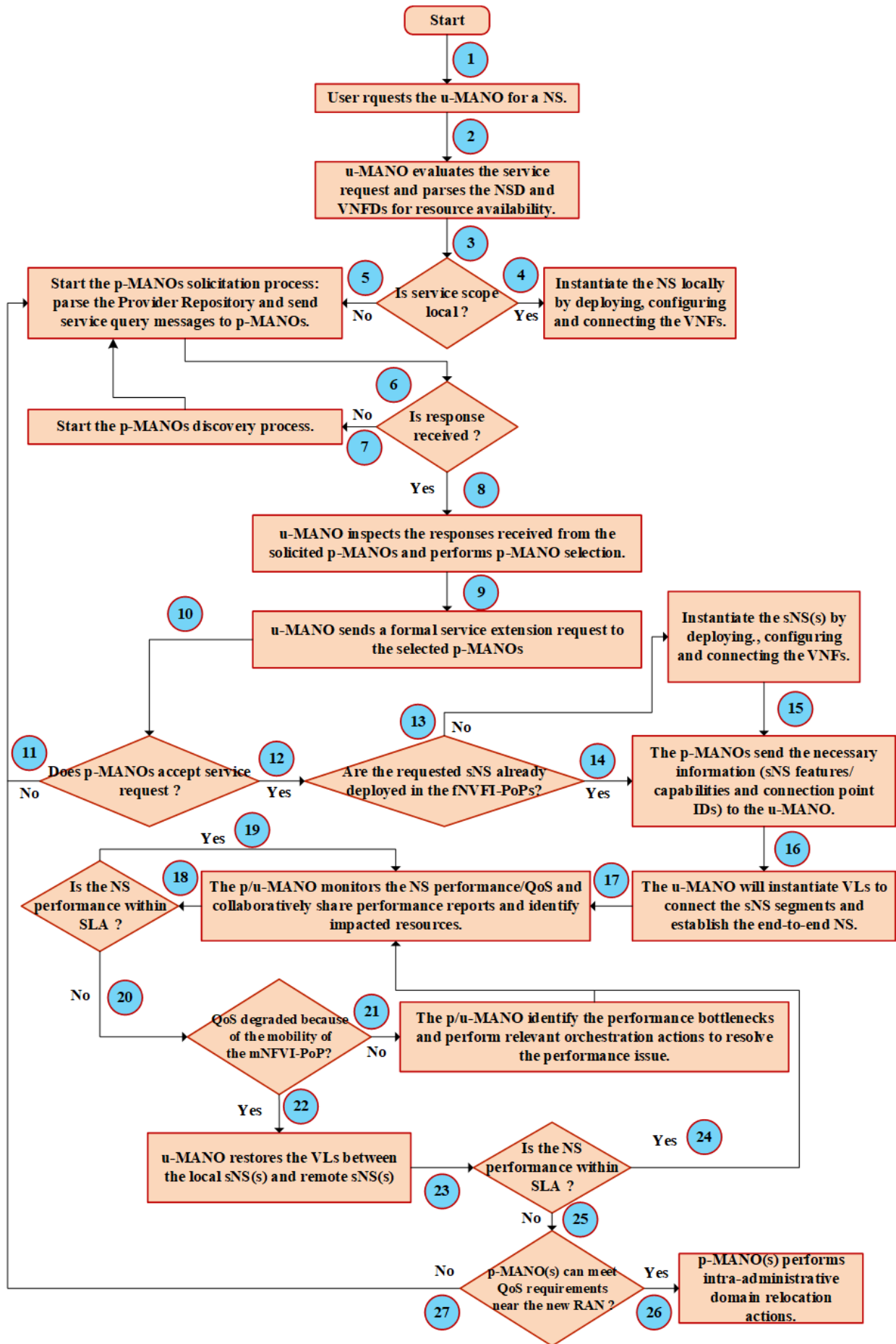
Fig. 4. Process Overview.
