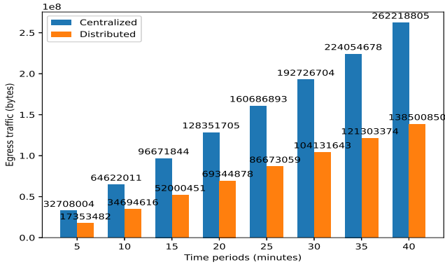
(a) Egress traffic measurements.
