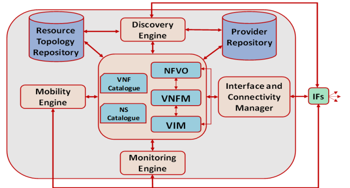
Fig. 3. u-MANO Functional Architecture.
