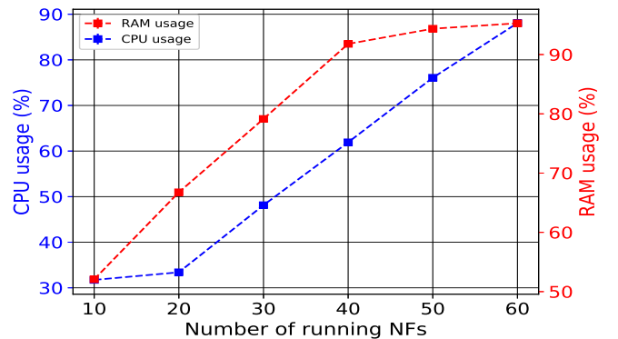
Fig. 5. u-MANO resources consumption.
