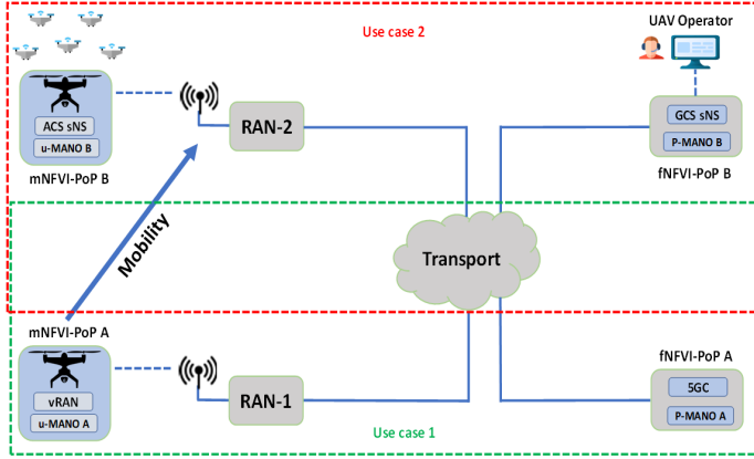
Fig. 1. Overview of the problem space.
