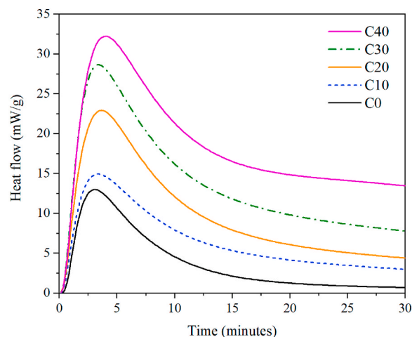
Fig. 3. Impacts of CSABF cement content on the dissolution peak and early ettringite precipitation of in situ mixed pastes (w/c = 0.5) at 23 °C.
