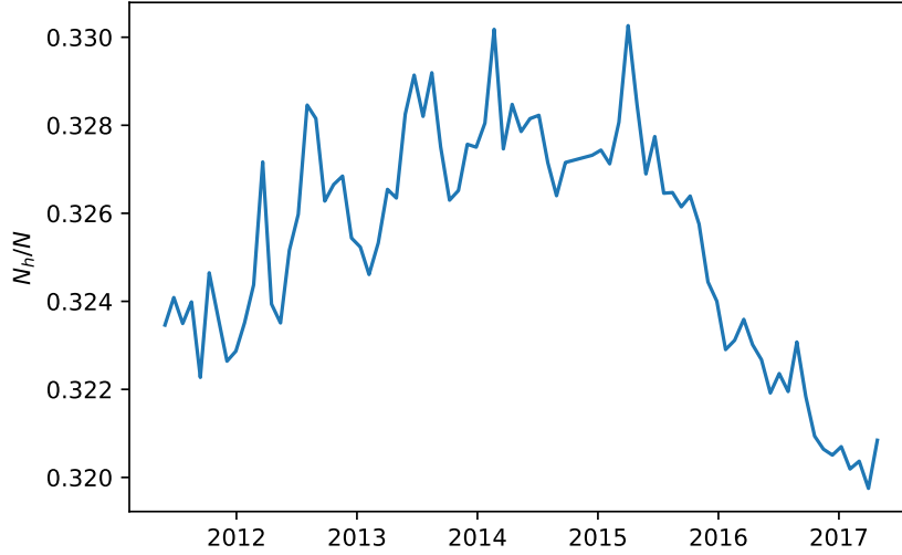
Figure 2: Contribution of heavy nuclei into the polar sea-level ( P_c=0.1 GV, d=1033 g/cm 2 ) NM response as a function of time obtained using direct observational data from the AMS-02 experiment.
