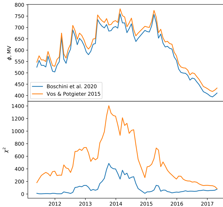
Figure 4: Solar modulation potential \phi (upper panel) and the corresponding quality of the best fit \chi^2 (lower panel) as obtained for AMS-02 data using two LIS models: Vos & Potgieter 2015 [9] (orange line) and Boschini et al. 2020 [16] (blue line).
