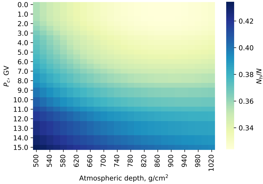
Figure 1: The relative contribution of heavy nuclei into the NM response as a function of cutoff rigidity P_c and atmospheric depth as obtained using the AMS-02 experimental data for BR 2462.
