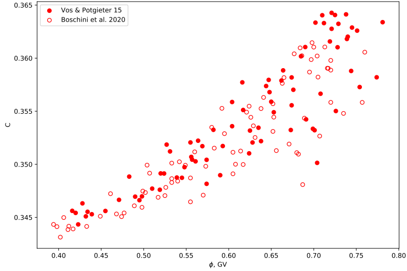
Figure 3: Dependence of the ratio C = N_{h,AMS}(\phi)/N_{h,mod} on the modulation potential \phi considering two LIS models: Vos & Potgieter 2015 [9] (full dots) and Boschini et al. 2020 [16] (empty dots).
