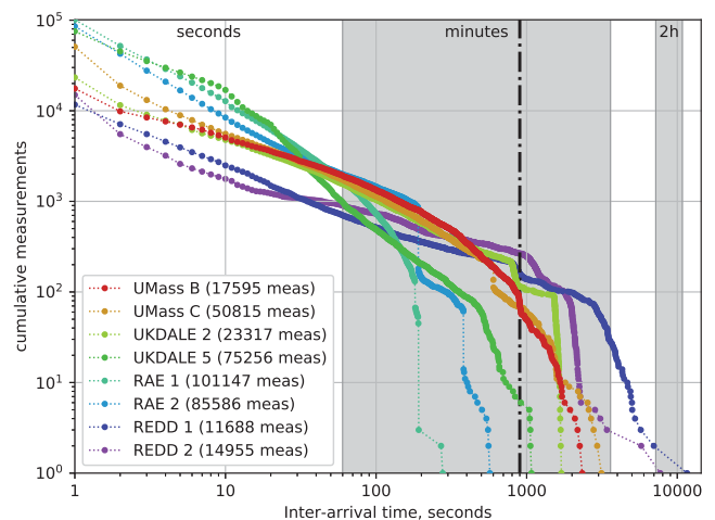
Fig. 4. Inter-arrival times for all houses, \Delta P = 10W . Vertical dashed line marks T=900s
