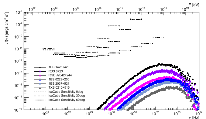
Figure 11. The maximum neutrino flux expected from the proton synchrotron model applied to six EHBLS. The IceCube sensitivity (IceCube Collaboration et al. 2019) for three different declinations is also represented.
