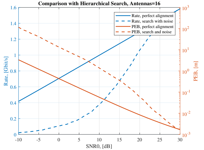
Figure 3. Comparison on the achievable rate (left axis) and position error bound (right axis) of hierarchical search strategy with perfect and imperfect beam-channel alignment. Number of antenna elements on BS and MS is equal N = M = 16 .
