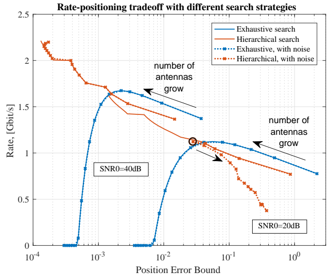
Figure 5. Rate as function of position error bound and number of antenna elements on BS and MS N = M . The black arrow indicating the direction in which the number of antennas is growing.
