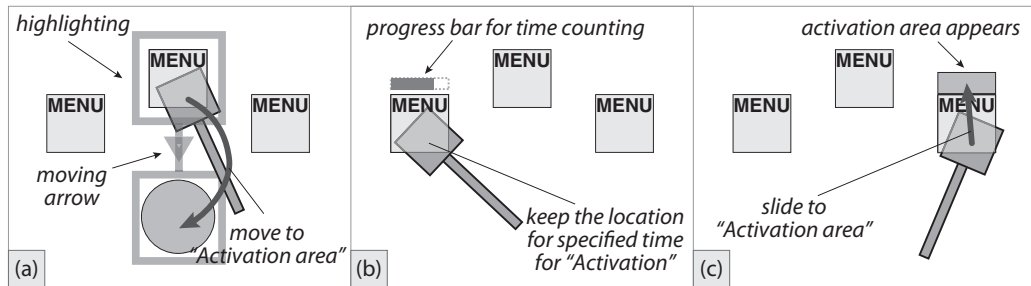
Fig. 2 Selection methods; (a) two-step, (b) hover, (c) slide.
