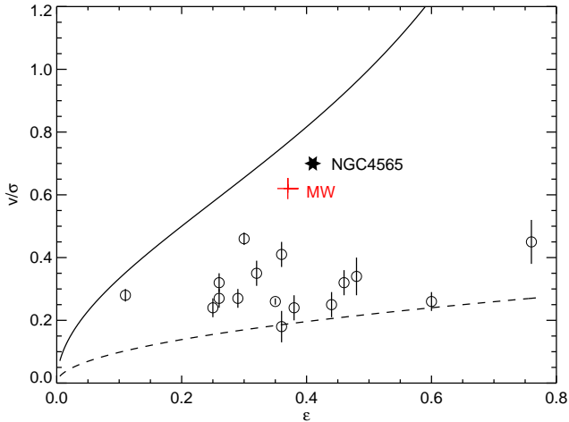
Fig. 17. Sixteen barlens galaxies common with Méndez-Abreu et al. (2018) and this work are shown in the V/\sigma - \epsilon plane. The parameters refer to values measured within one R_e of the bulge (see Table 2 in Méndez-Abreu et al. 2018). They are corrected for pixelation and resolution effect (as explained in the original paper). The solid line shows the expected relation for rotationally flattened spheroids seen edge-on, following the approximation V/\sigma = \sqrt{\epsilon/(1-\epsilon)} given in Kormendy (1982). The dashed line ( V/\sigma = 0.31 \sqrt{\epsilon} ) shows the region in which the slowly rotating bright ellipticals fall in the study by Emsellem et al. (2011; see their Fig. 6a). Also indicated in the figure are the Milky Way (MW) bulge (red cross) and NGC 4565 (star) using the values from Rich et al. (2008).
