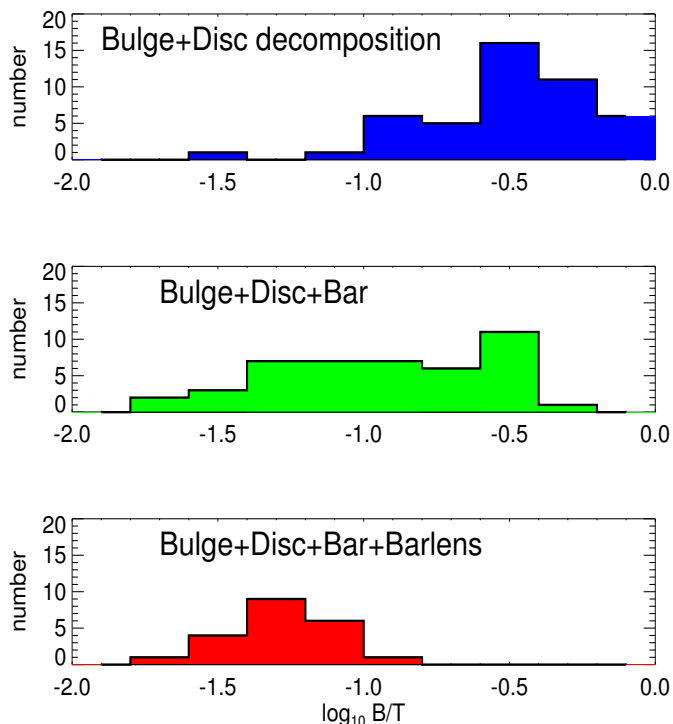
Fig. 5. Bulge-to-total ( B/T ) flux ratios for the 46 galaxies decomposed in this study. The values in three type of models are shown: bulge/disk (B/D, upper panel ), bulge/disk/bar (B/D/bar, middle panel ) and bulge/disk/bar/bl (B/D/bar/bl, lower panel ). The B/T values for the individual galaxies are shown in Table 1. Compared to the B/D and B/D/bar models, the number of the B/D/bar/bl models is smaller because only half of the decomposed galaxies were fitted with a separate bulge component
