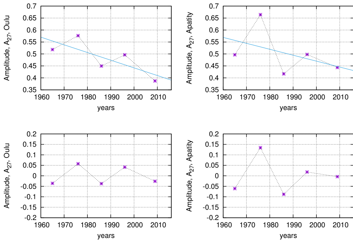
Fig. 2. Three-year means of amplitude of the first ( A_{27} ) harmonic of GCR for the last five solar minima with linear trend (upper panels) and detrended (lower panels) for the Oulu (left panels) and Apatity (right panels) neutron monitor count rates.
