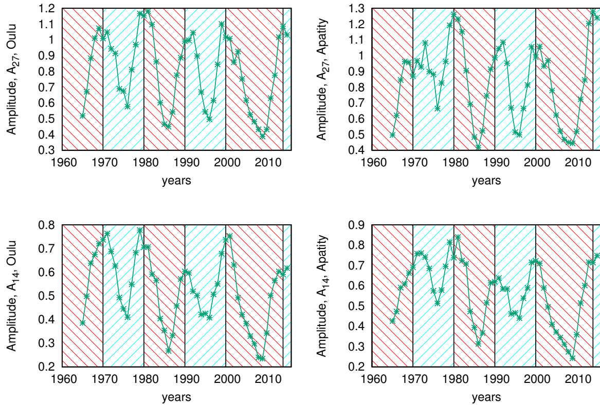
Fig. 1. Three-year running means of yearly averaged amplitudes of the first ( A_{27} , upper panels) and the second ( A_{14} , lower panels) harmonics of GCR for the Oulu (left panels) and Apatity (right panels) neutron monitor count rates in 1964–2016 during A > 0 epochs (cyan boxes with upward lattice) and A < 0 epochs (red boxes with downward lattice).
