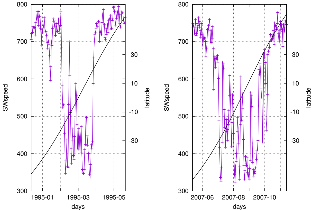
Fig. 4. Daily SW speed measured by Ulysses during the first (12.1994–05.1995, left panel ) and the third (05.2007–11.2007, right panel ) fast latitudinal scan. The black dash-dotted curve ( y -axis on the right) illustrates the latitudinal position of the space probe during that period.
