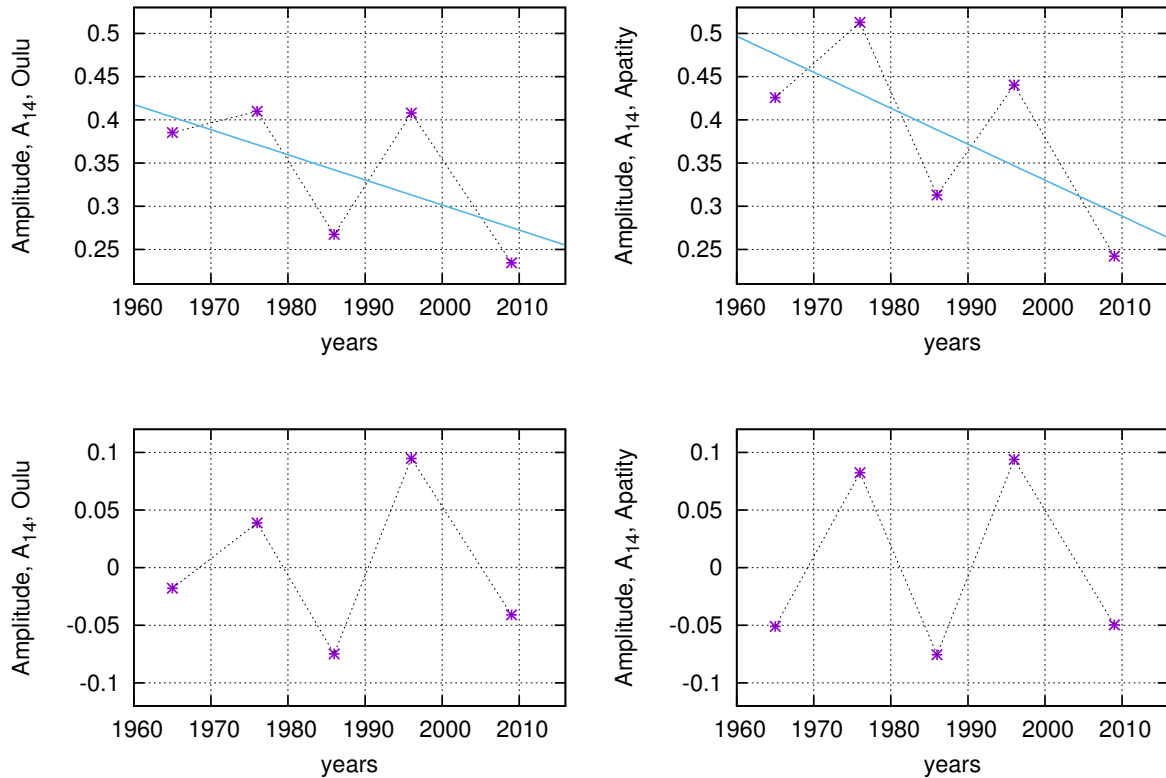
Fig. 3. Three-year means amplitude of the second ( A_{14} ) harmonic of GCR for the last five solar minima with linear trend ( upper panels ) and detrended ( lower panels ) for the Oulu ( left panels ) and Apatity ( right panels ) neutron monitor count rates.
