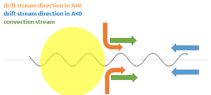
Fig. 5. Directions of convection and drift during A > 0 and A < 0 (adapted from Moraal & Mulder 1985).
