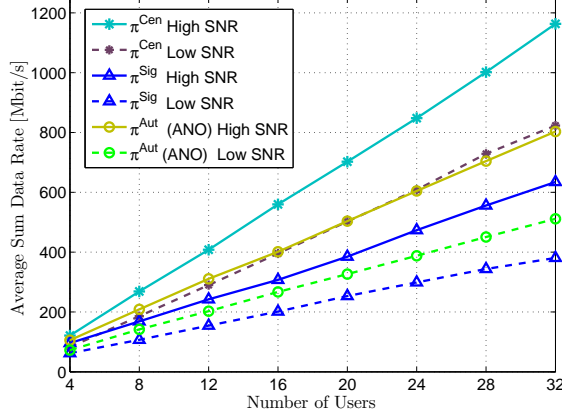
Fig. 9: Average sum data rate vs. number of users I for the \pi^{Aut} , \pi^{Sig} and the \pi^{Cen} methods. Number of subchannels is increased with the number of users, i.e., |\mathcal{S}_p| = I .
