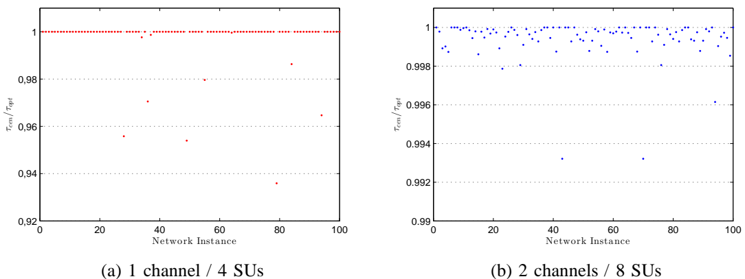
Fig. 3: Ratio of time average data rate of the \pi^{Cen} subchannel assignment to the optimal assignment.
