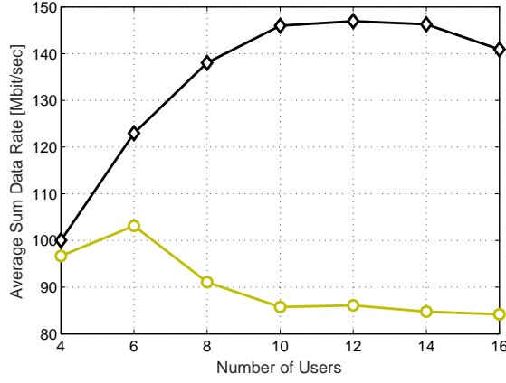
Fig. 7: Average sum data rate achieved by the \pi^{Aut} under the APS and ANO CB selections as a function of Number of users I , where |\mathcal{S}_p| = 8 , and ACI = 5\% . Users are with heterogeneous CB capabilities. i.e, maximum CB capabilities are uniformly selected from O_{max,i} = 1 to O_{max,i} = |\mathcal{S}_p| .
