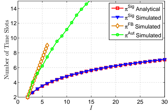
Fig. 4: Expected time to converge to conflict free subchannel selections of the \pi^{Sig} and \pi^{FB} methods as a function of I users, under collision-protocol model. The number of available subchannels |\mathcal{S}_p| = I , and O_{max,i} = 1\forall i .
