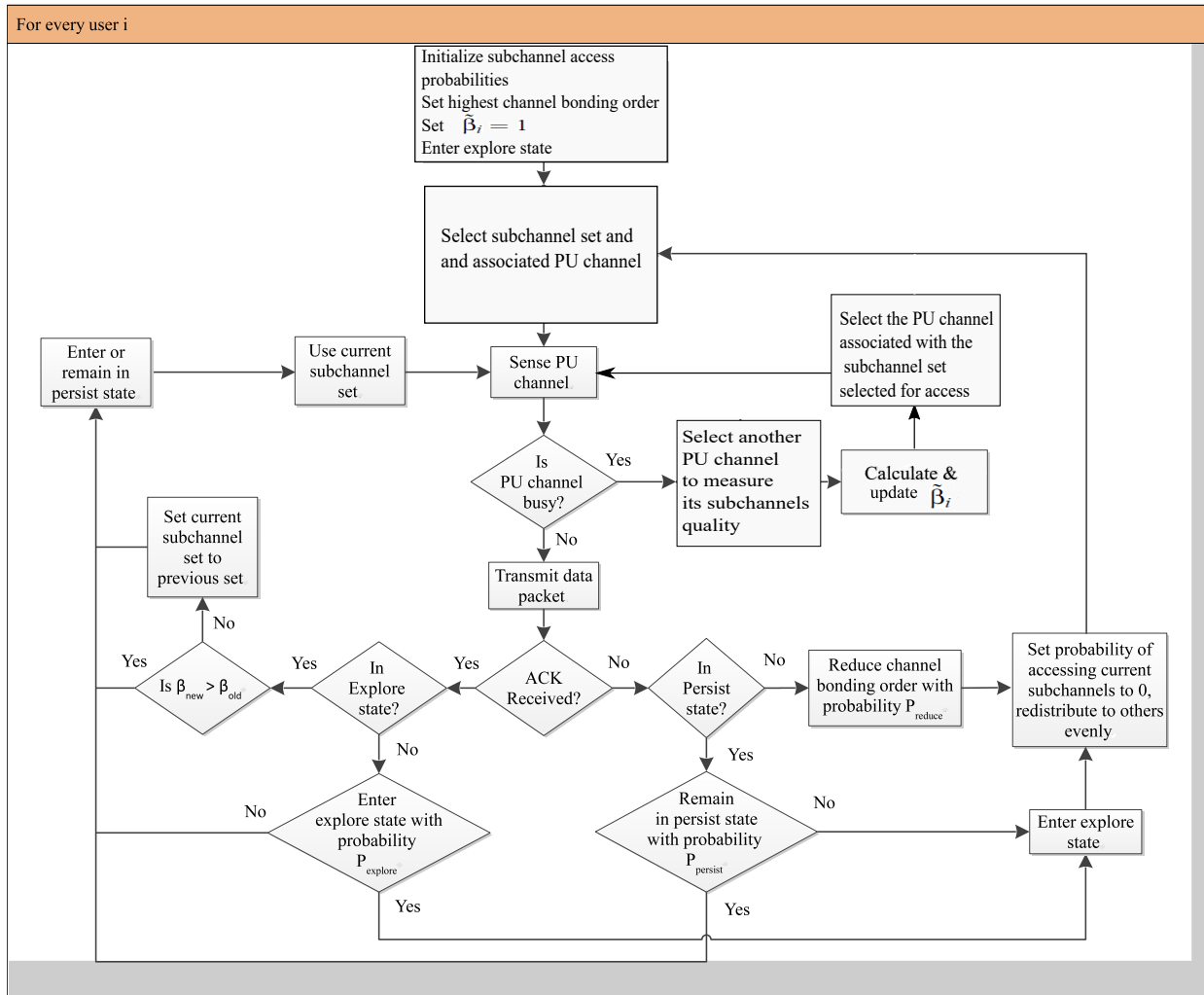
Fig. 2: \pi^{Aut} Method.
