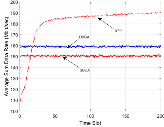
Fig. 6: Average sum data rate vs. time for the proposed \pi^{Aut} method, SBCA and DBCA, where |S_p| = 8 , N_R = 50m , and I = 8 users, with maximum CB capability of bonding 3 subchannels.
