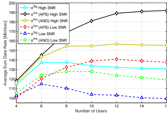
Fig. 5: Average sum data rate achieved by the \pi^{Aut} and \pi^{Sig} methods vs. number of users, with |\mathcal{S}_p| = 8 , N_R = 50meters , and users with heterogeneous CB capabilities, i.e, maximum CB capabilities are uniformly selected from O_{max,i} = 1 to O_{max,i} = |\mathcal{S}_p| .
