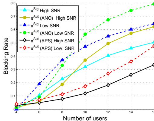
Fig. 10: User blocking rate of the \pi^{Aut} and \pi^{Sig} methods as a function of Number of users I . with ANO selections method, when the number of users is less than 16 in the high SNR case, and 10 in the low SNR case. However, its blocking rate is higher than the \pi^{Aut} with APS selections method. For an increased number of users, i.e. as the ratio of users to subchannels increases, the blocking rate of the \pi^{Aut} method under both ANO and APS selections is lower than the \pi^{Sig} method. This shows that the information provided by the SAS (under the assumption of collision domain model) to users in the \pi^{Sig} method is useful for reducing conflict between users when the ratio of users to useable subchannels is suitably low. When the ratio of users to subchannels increases, it becomes increasingly likely that all subchannels are determined by the SAS to be in a state of conflict (i.e. state 0), therefore the subchannel status bit-maps no longer contain any useful information. In reality two or more users within interference range of one another may select the same subchannel, with interference levels low enough not to cause a collision. It is for this reason that the limited feedback information utilized in the \pi^{Aut} method proves to be more beneficial as the ratio of users to subchannels grows large.
