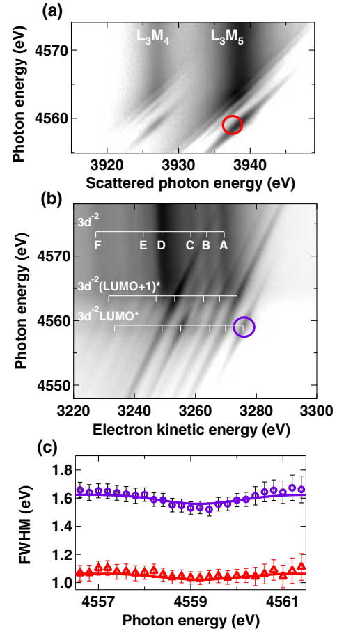
FIG. 1. (a) RIXS L_3M_{4,5} and (b) Auger L_3M_{4,5}M_{4,5} spectra recorded in \text{CH}_3\text{I} near the I L_3 edge. A detailed assignment of the labeled Auger lines is presented in the Supplemental Material [30]. (c) FWHM of RIXS emission line (triangles) and Auger line (circles) selected in (a) and (b), respectively, as a function of photon energy around the LUMO resonance. Error bars are obtained from the fits of the experimental spectra. Solid lines show simulations based on Eqs. (2) and (3).
