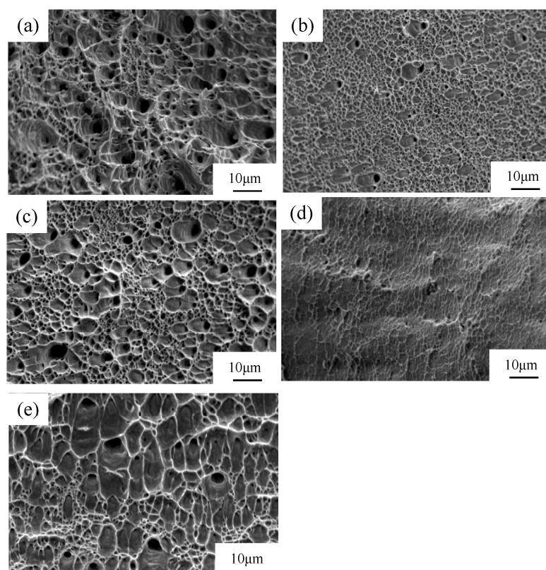
Figure 6. Fracture surface morphology of the 316LN austenitic stainless steel before and after rolling: (a) original austenite structure; (b) CR-30%; (c) RTR-30%; (d) CR-90%; and (e) RTR-90%.
