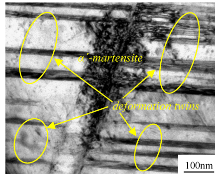
Figure 7. Martensite formed at the interaction position of deformation twins.
