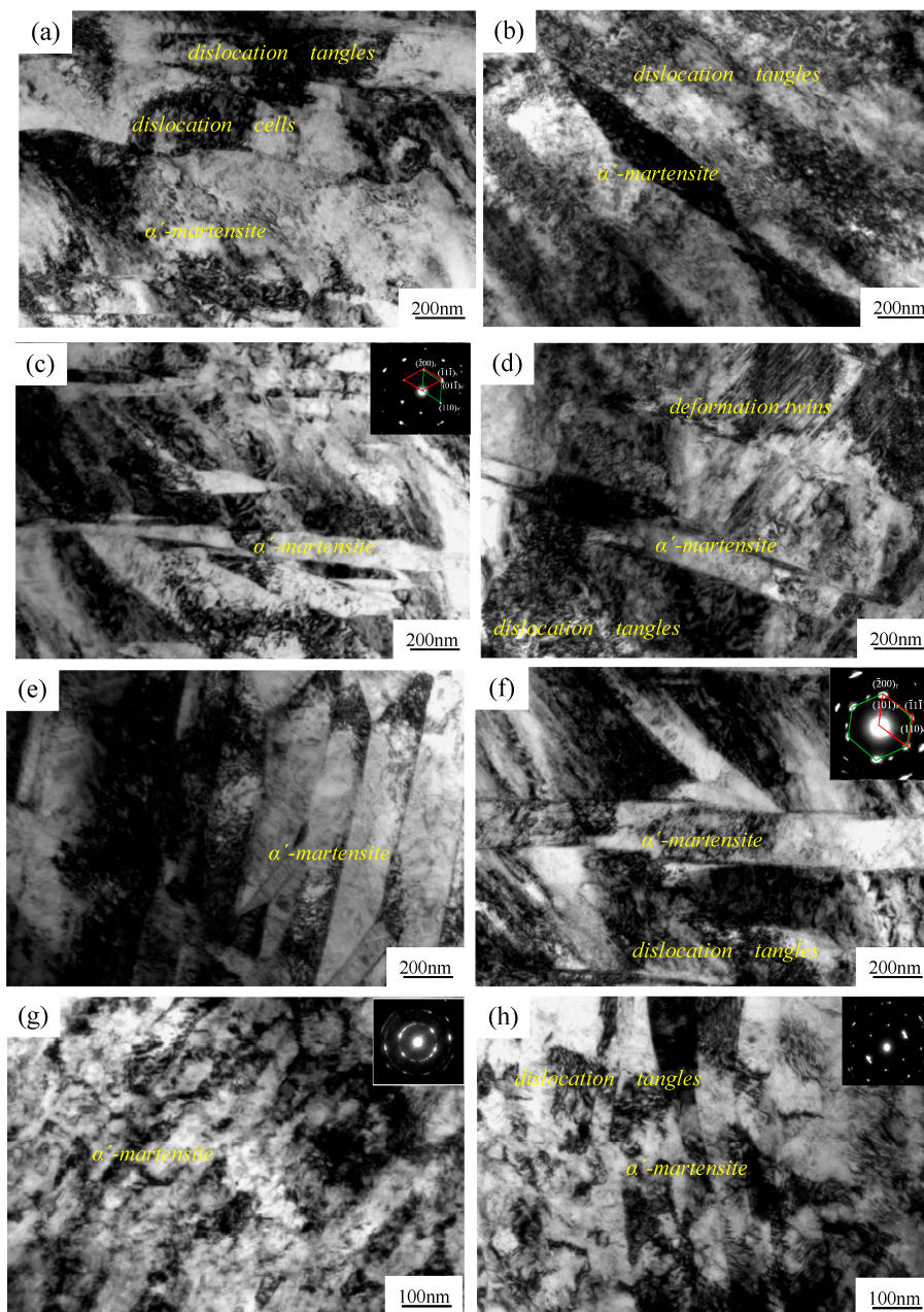
Figure 4. TEM images of the 316LN austenitic stainless steel after CR and RTR: (a) CR-30%, (b) RTR-30%, (c) CR-50%, (d) RTR-50%, (e) CR-70%, (f) RTR-70%, (g) CR-90%, and (h) RTR-90%.
