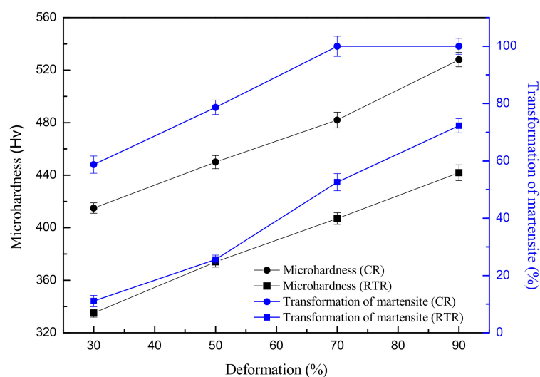
Figure 2. Relationship of the volume fraction of the martensite and microhardness with deformations at different temperatures (the data of CR is from [14]).
