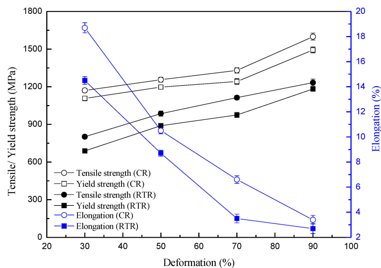
Figure 5. Relationship of the strength and elongation with deformations at different temperatures (the data of CR is from [14]).
