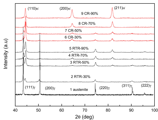
Figure 1. XRD patterns of the 316LN austenitic stainless steel before and after deformation at different temperatures (the data of CR is from [14]).
