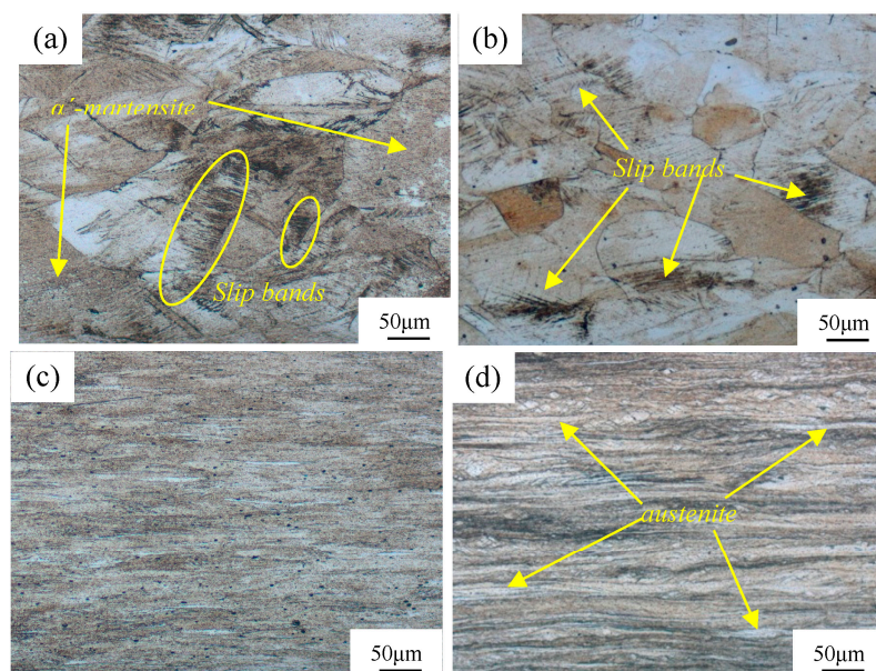
Figure 3. Metallographic structure of the 316LN austenitic stainless steel after CR and RTR: (a) CR-30%, (b) RTR-30%, (c) CR-90%, and (d) RTR-90%.
